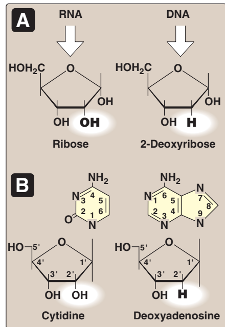
Figure 22.3 A. Pentoses found in nucleic acids. B. Examples of the numbering systems for purine- and pyrimidine-containing nucleosides.
