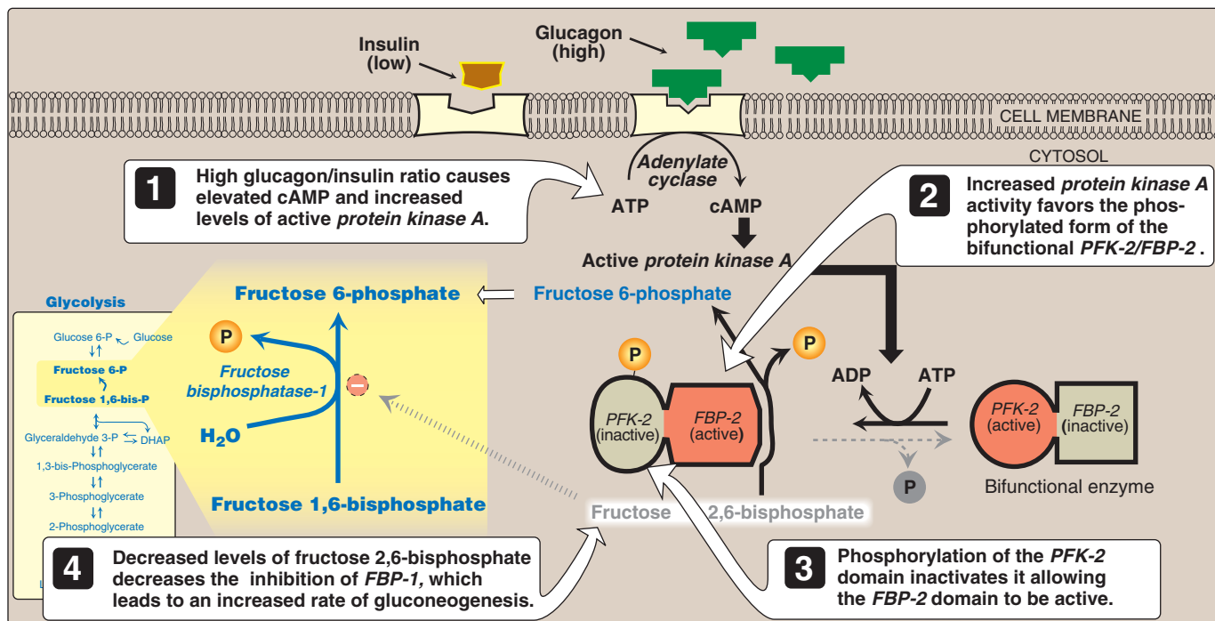
Figure 10.5 Effect of elevated glucagon on the intracellular concentration of fructose 2,6-bisphosphate in the liver. PFK-2 = phosphofructokinase-2; FBP-2 = fructose bisphosphatase-2.
