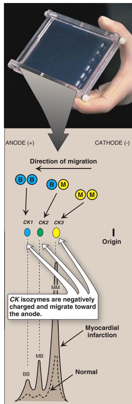
Figure 5.21 Subunit structure, electrophoretic mobility, and enzyme activity of creatine kinase ( CK ) isoenzymes.
