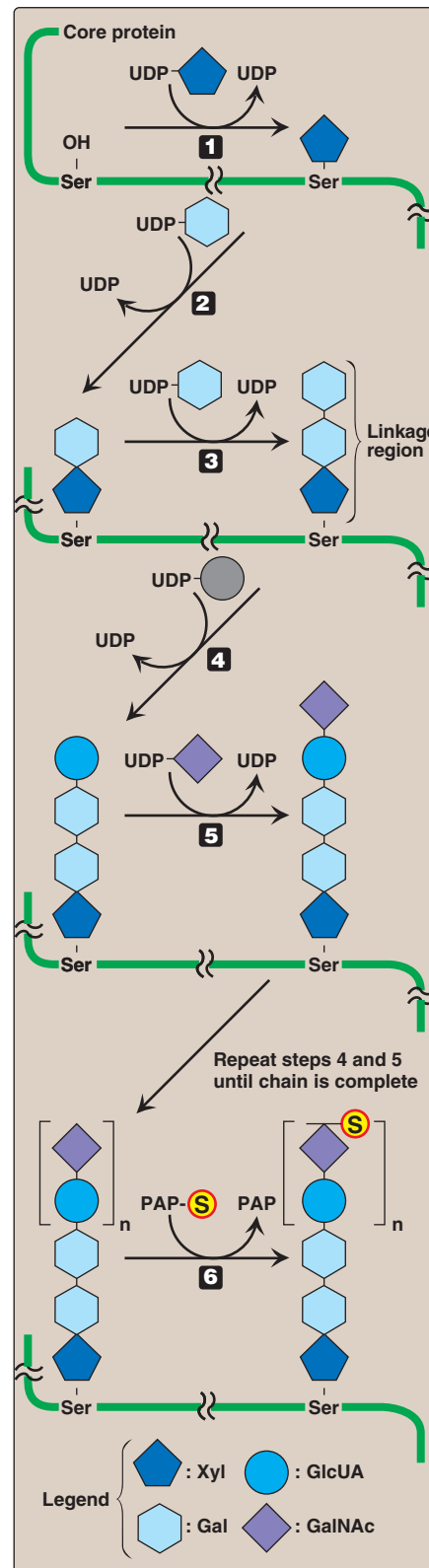
Figure 14.11 Synthesis of chondroitin sulfate.
